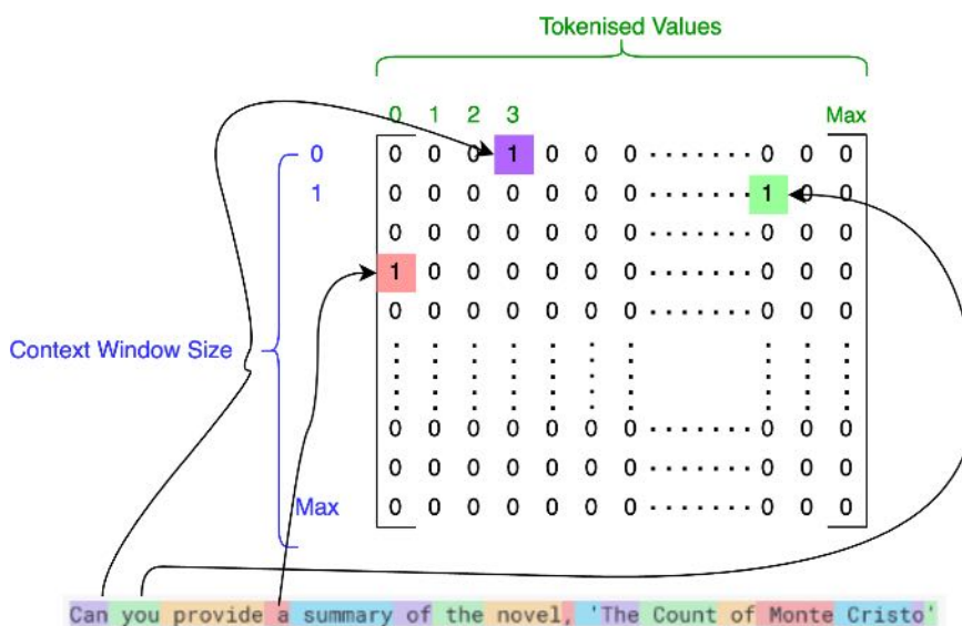
Figure 6.15 Encoding Matrix.
