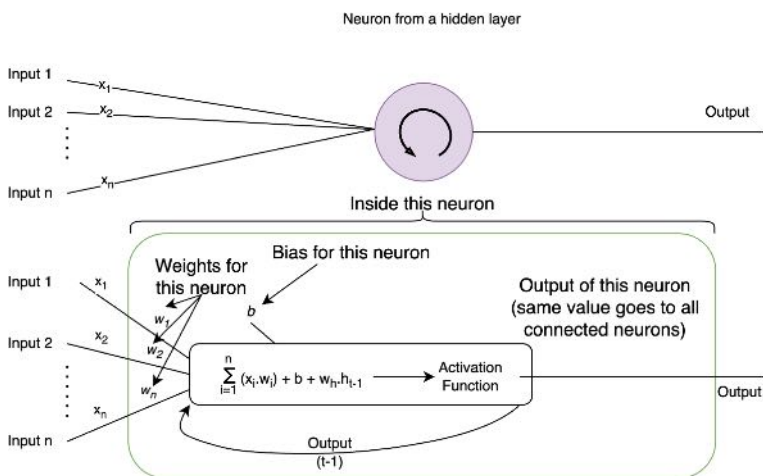
Figure 6.10 Recurrent Cell.
