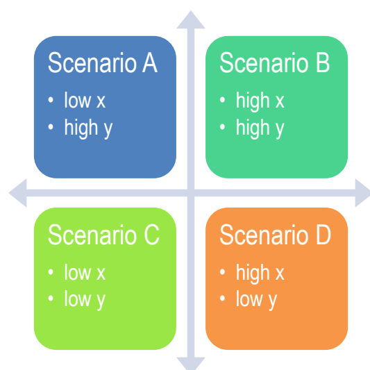
Figure 3. Simplified 2x2 scenario matrix using critical uncertainties x and y
