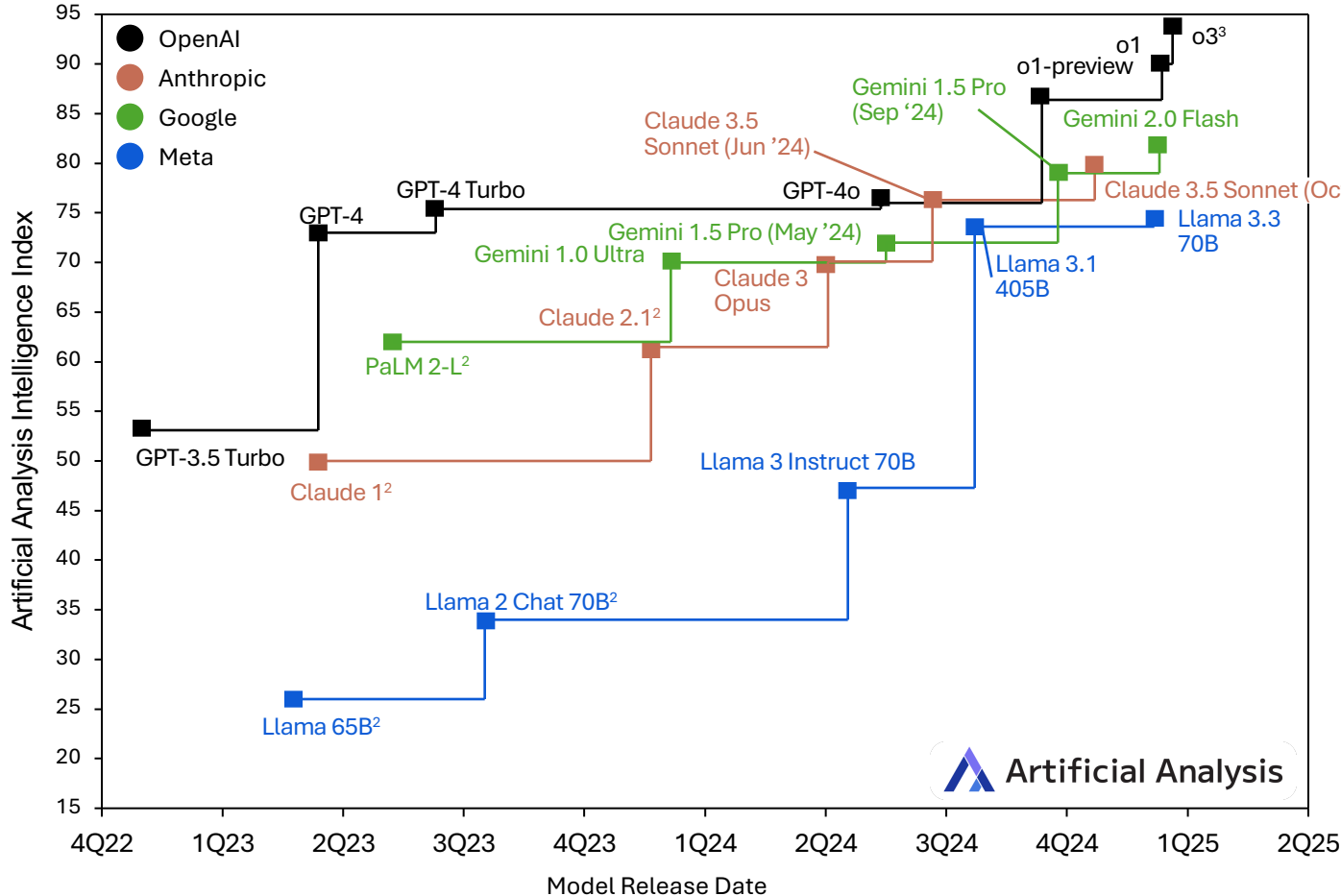
Artificial Analysis Intelligence Index: MMLU, GPQA Diamond, MATH-500, HumanEval. Top 5 Labs by Market Share.
