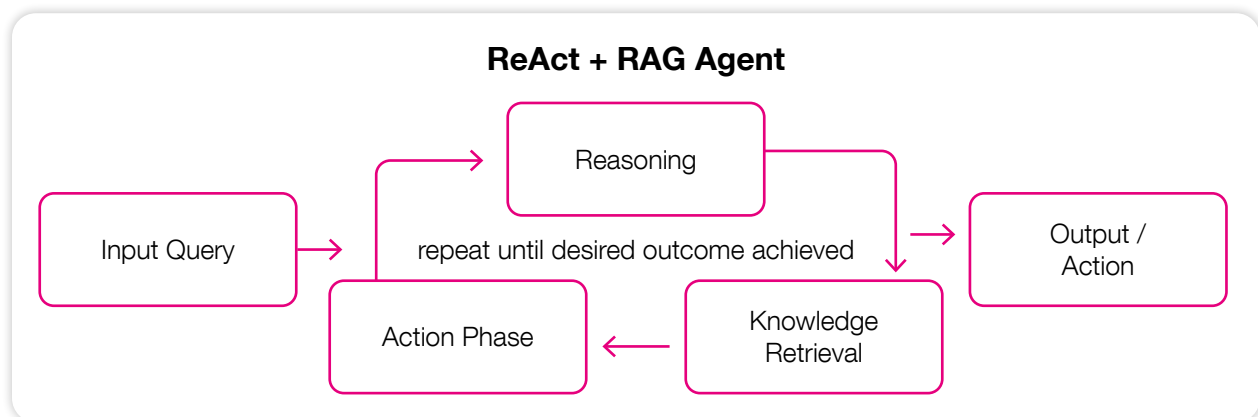
Fig 1.5: Workflow of a ReAct + RAG agent
