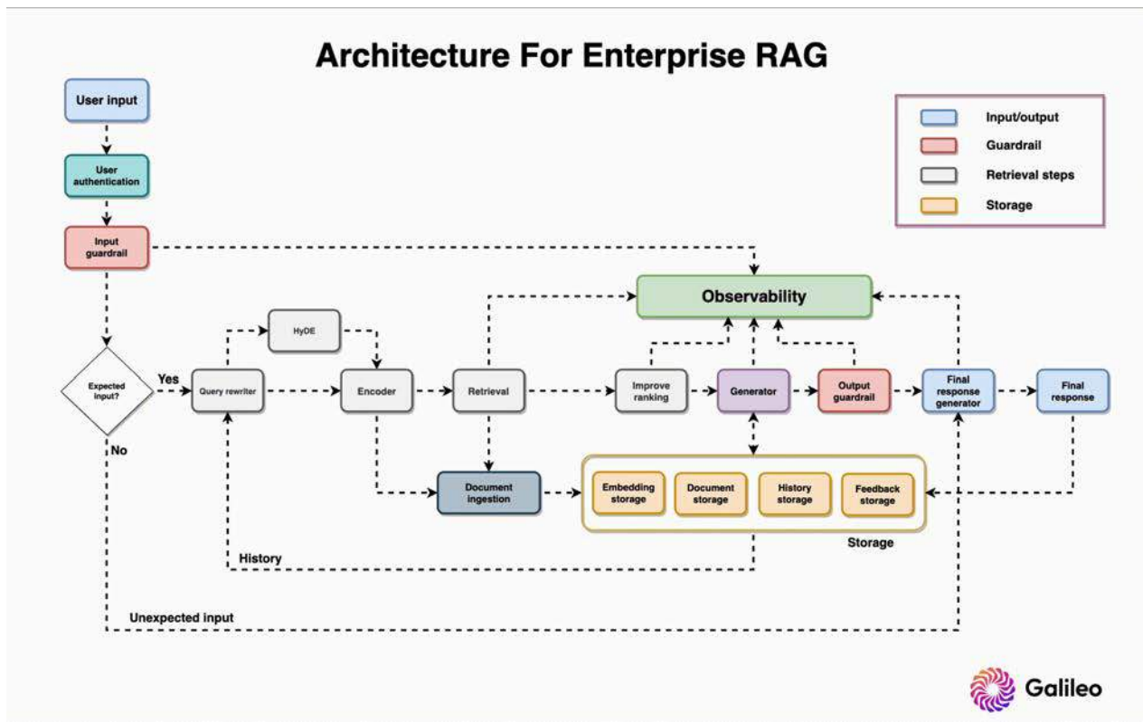
Fig 7.2: Enterprise RAG architecture
