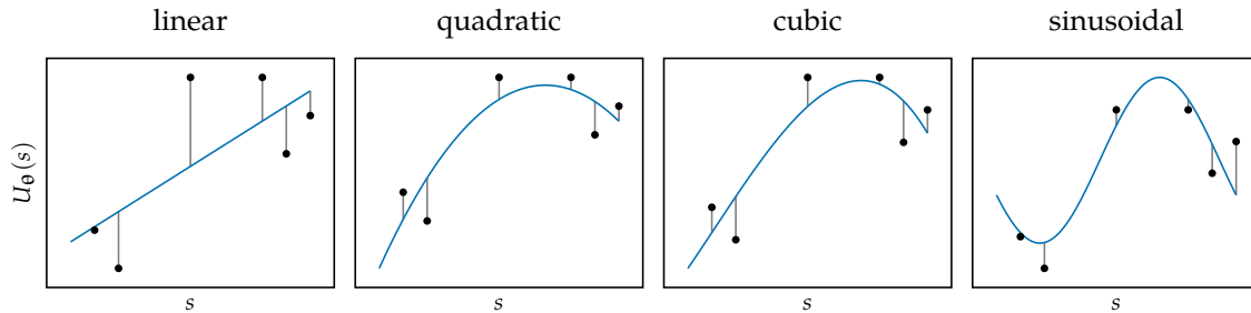
Figure 8.13. Linear regression with different basis function families.
