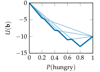
Figure 21.6. The sawtooth upper bound representation applied to the crying baby problem.
