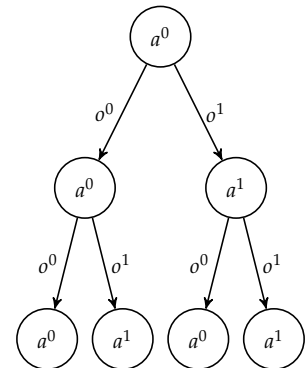
Figure 20.1. A three-step conditional plan.
