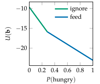
Figure F.10. The optimal policy for the crying baby problem. This infinite horizon solution does not recommend singing for any belief state. As shown in figure 20.3, it is optimal to sing in some finite-horizon versions of this problem.
