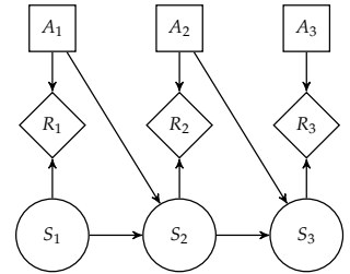
Figure 7.1. MDP decision network diagram.
