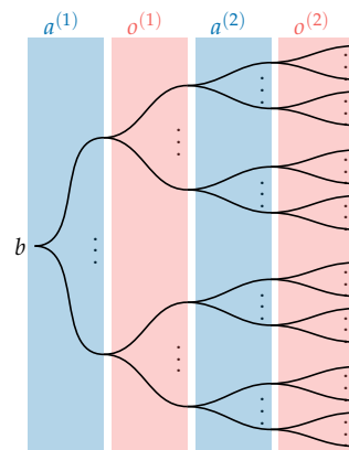
Figure 22.1. Forward search searches the action-observation-belief graph to an arbitrary finite depth in order to select the action that produces the highest expected reward. This illustration shows a search to depth 2.
